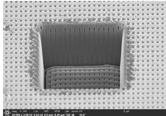
Rectangular box milled into a semi-processed vertical NAND memory
